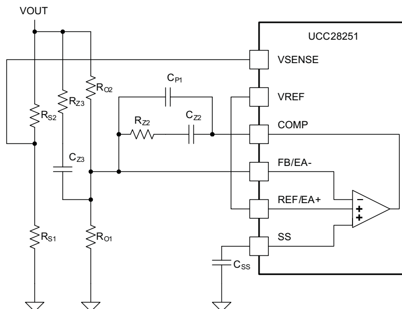
Figure 41. Error Amplifier Set Up for Secondary-Side Control
