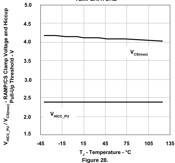
RAMP/CS CLAMP VOLTAGE AND HICCUP PULL-UP THRESHOLD VS TEMPERATURE
