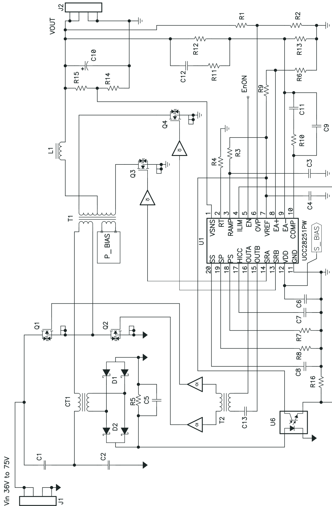
Figure 2. Secondary-Side Half-Bridge Controller with Synchronous Rectification
