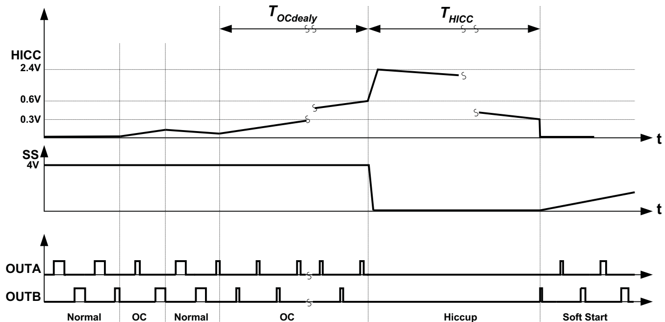
Figure 46. Cycle-by-Cycle Current Limit Delay Timer and Hiccup Restart Timer
