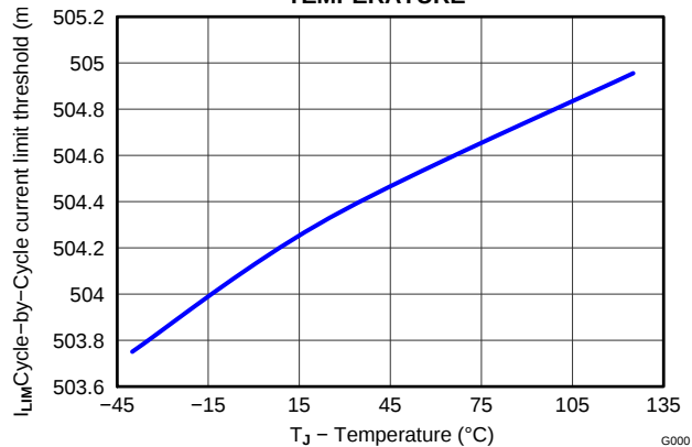
CYCLE-BY-CYCLE CURRENT LIMIT VS TEMPERATURE
